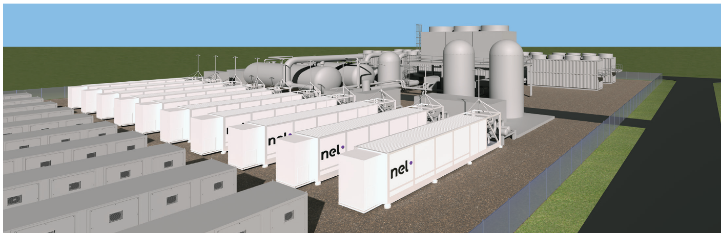
100 MW PEM electrolysis plant featuring ten PSM containerized modules.
